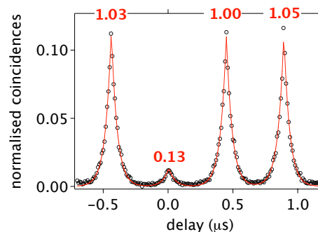
Fig. 3. Histogram of time intervals between consecutive photodetection events in the two paths of the wavefront-splitting interferometer. The pulsed excitation laser repetition period is 444 ns, and the total counting time was 148.15 s. Lines are exponential fits for each peak, corresponding to a radiative lifetime of 44.6 \pm 0.8 ns. Values written above each peak correspond to their respective area normalized to the corresponding value for Poissonian photon number statistics. The strong reduction of coincidences around zero delay gives evidence for single-photon emission by the excited N-V colour centre and for its particle-like behaviour as the wavefront is split in two parts by the Fresnel’s biprism.
